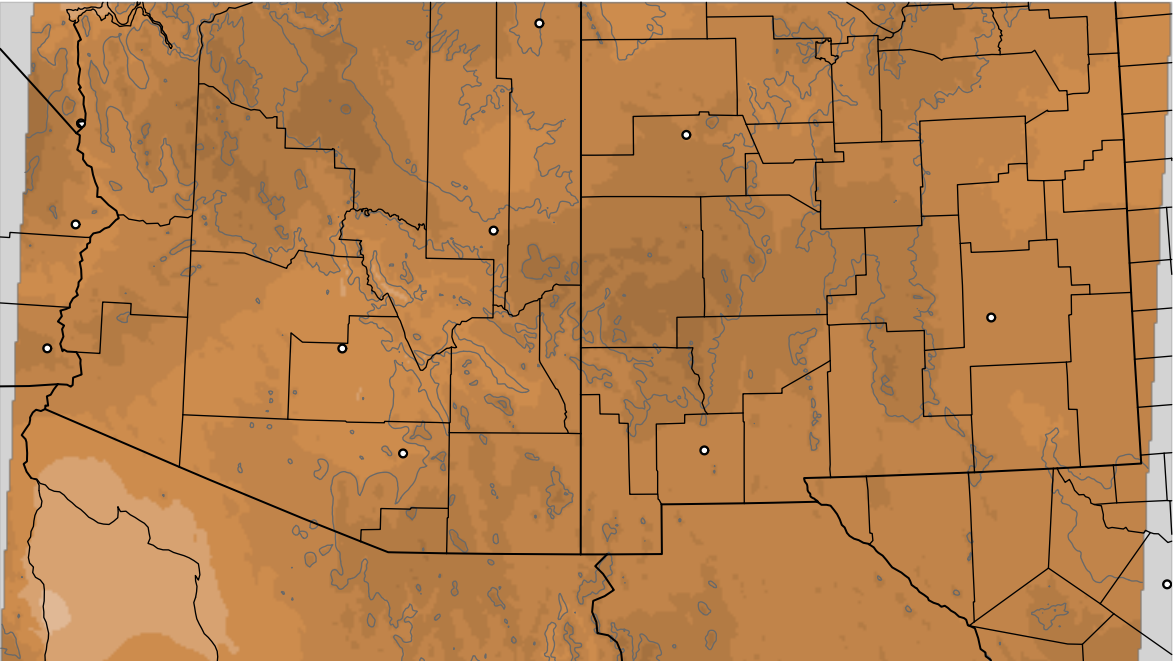
Corrected PWV 24 Mar 2019 11:45 UTC
