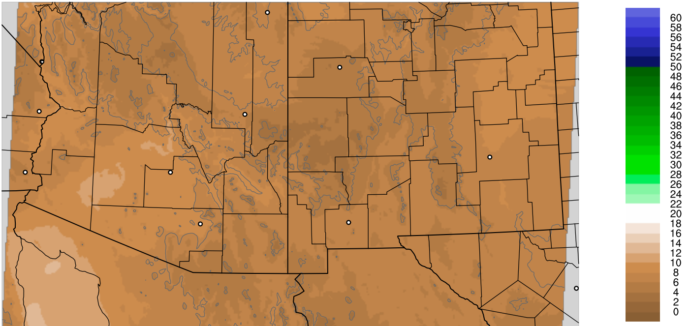
Corrected PWV 24 Mar 2019 11:45 UTC
