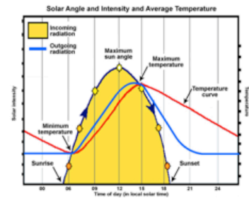
Black curve-incoming solar radiation Blue curve-outgoing IR radiation Red curve-temperature
