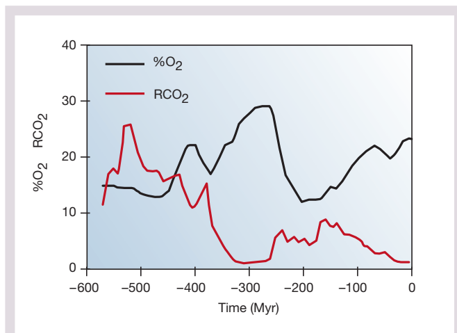
Figure 5 Plots of RCO 2 (the ratio of the mass of carbon dioxide in the atmosphere in the past to that for the pre-industrial present) and %O 2 during the Phanerozoic eon. (Values of RCO 2 from the GEOCARB III model 33 ; values of %O 2 from ref. 11 using the 13 C data of refs 12 and 13). Estimated errors are ±50% for RCO 2 and ±7% for O 2 .
