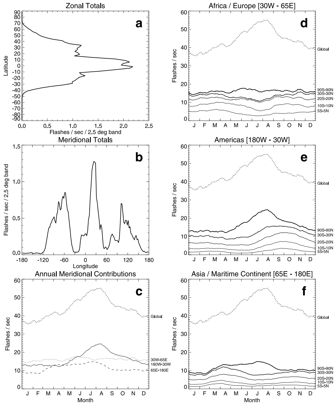
Figure 8. The annual cycle of global flash rate decomposed zonally and meridionally. (a) Zonal total flash rate in 2.5° latitude bands. (b) Meridional total flash rate in 2.5° longitude bands. (c) Meridional contributions corresponding roughly to the Americas, Europe and Africa, and Asia and the Maritime Continent. (d–f) Annual cycles for the three main land regions decomposed into their tropical and subtropical components.
