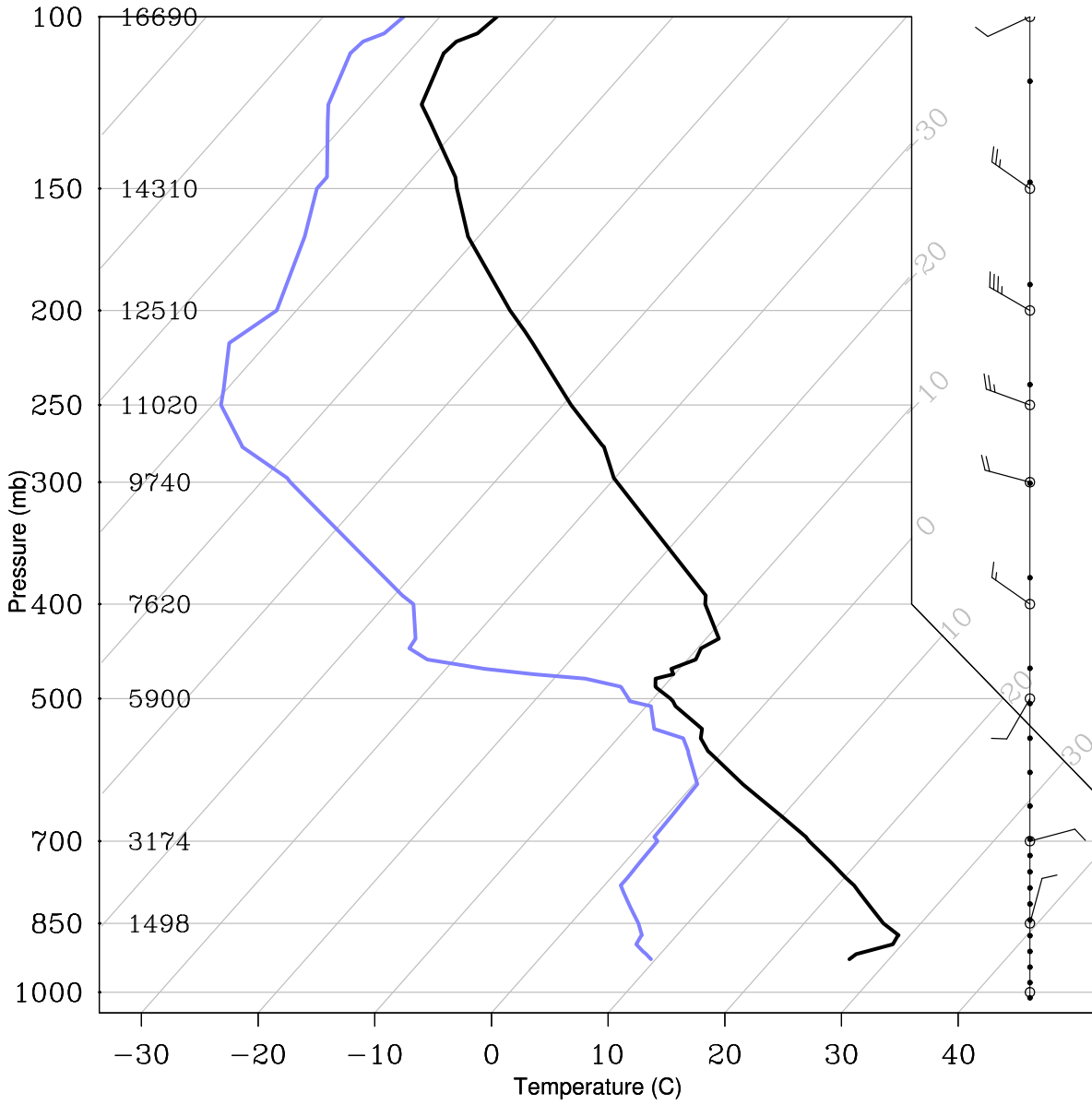
(Fig 3b) Tucson Skew-T, Sept 4, 2011 (00Z or 12Z)?
