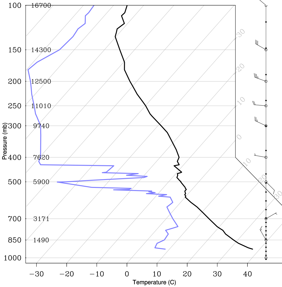
(Fig 3a) Tucson Skew-T, Sept 4, 2011 (00Z or 12Z)?
