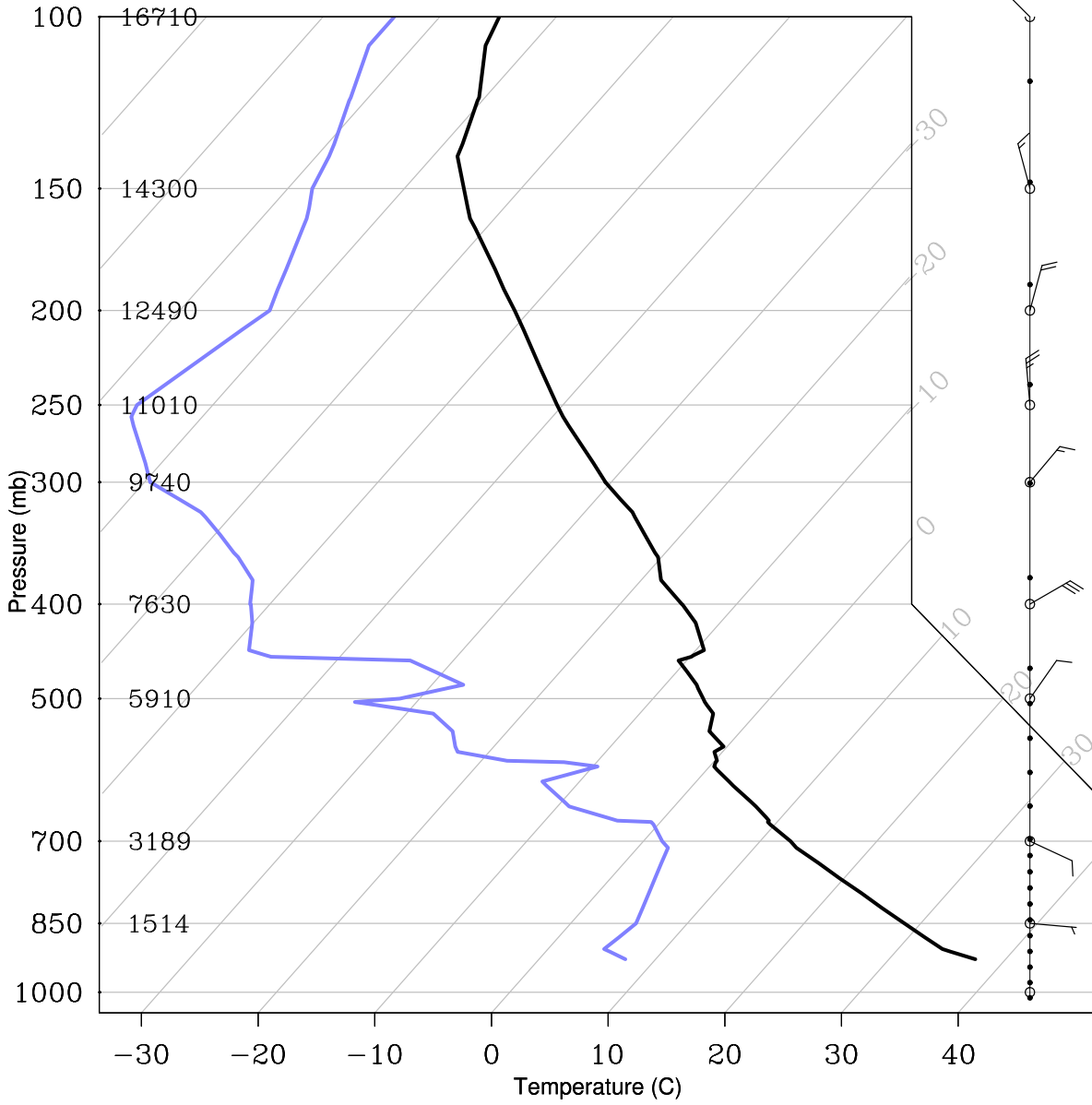
Tucson Skew-T, Sept 5, 2010 (00Z or 12Z)?
