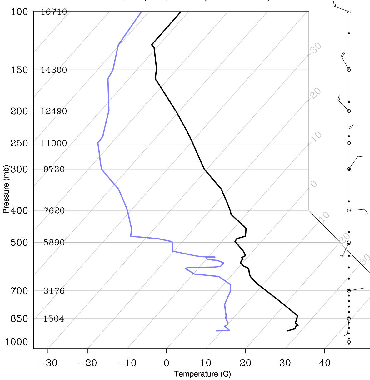
Tucson Skew-T, Sept 5, 2010 (00Z or 12Z)?
