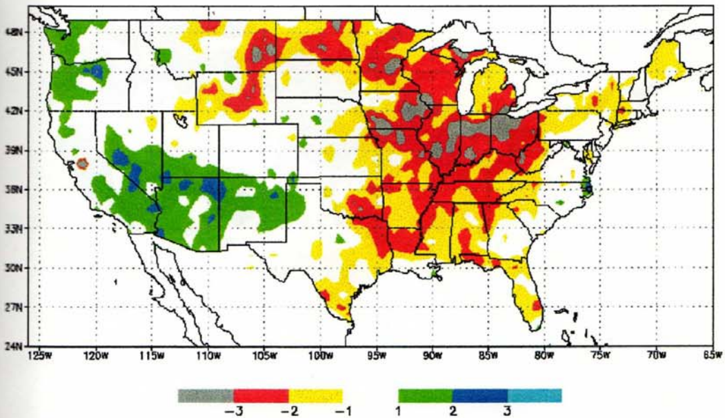
3 Month SPI: JUN 1988
