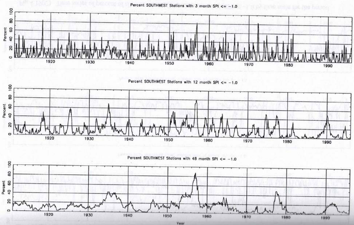
Fig 4. 19(D) Time series of percent of all Southwest stations with SPI \leq -1.0 by time scale for the period January, 1911 through December, 1993
