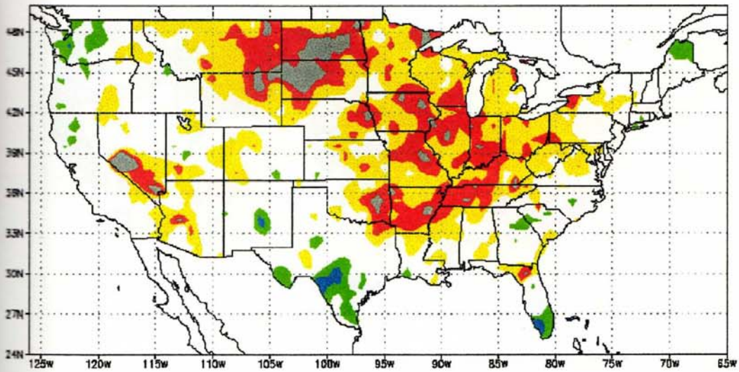
3 Month SPI: JUN 1936
