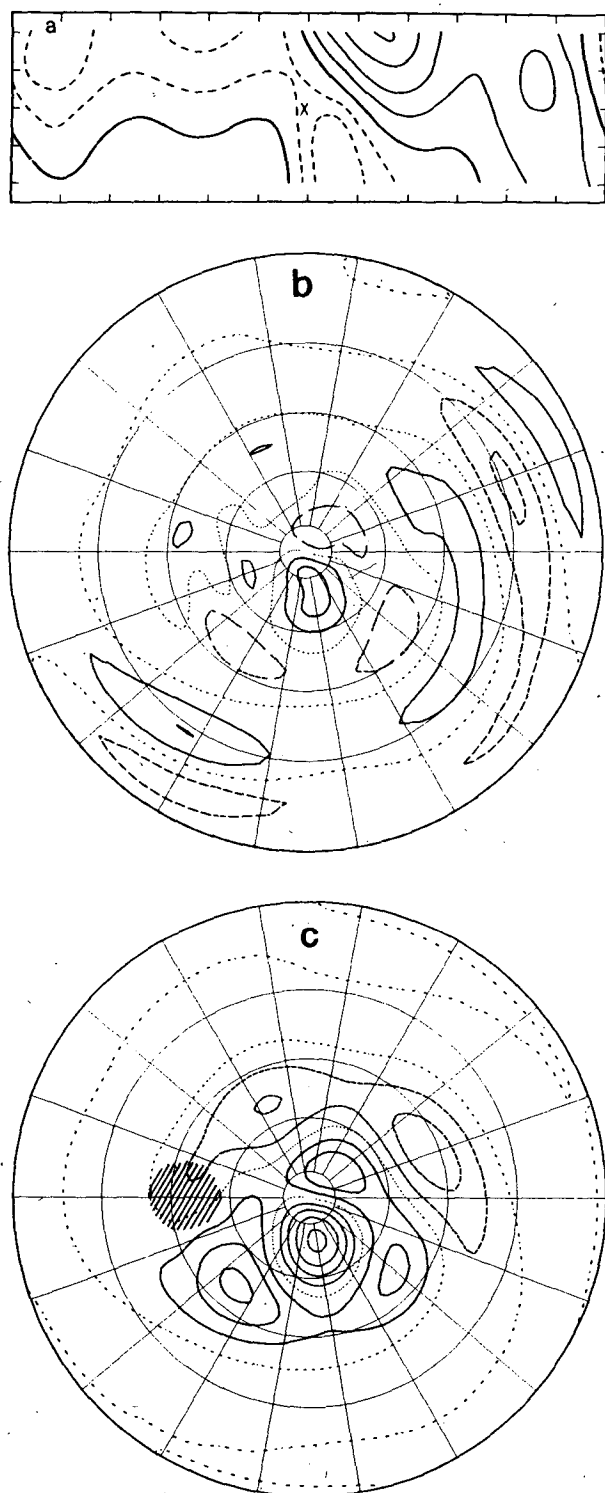
FIG. 4. Solution for a deep circular heat source at 45° using the NH winter flow. Shown are (a) height field in a longitude-height section at 46.0°N, (b) 300 mb vorticity perturbation, and (c) 300 mb height field perturbation. Contours as in Fig. 3, except that the contour interval in (a) is now 2 dam.
