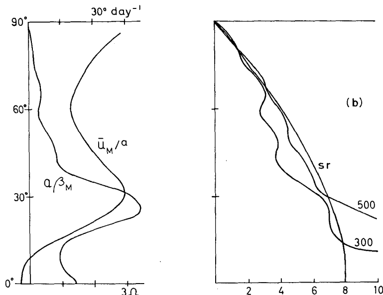
FIG. 13. (a) \bar{u}_M/a ( \text{deg day}^{-1} ) and \alpha/\beta_M for the 300 mb NH winter flow used in the model. (b) Stationary wavenumbers aK_s for the super-rotation flow, and the 500 and 300 mb NH winter flow.
