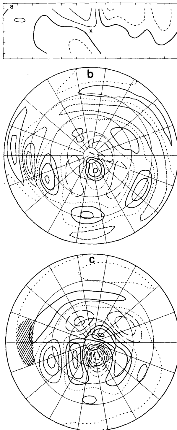
FIG. 3. Steady state, linear solution of a five-layer baroclinic model for a deep elliptical heat source at 15^\circ perturbing the Northern Hemisphere winter zonal flow. Shown are (a) height field in a longitude-height section at 18.1^\circ\text{N} (contour interval 1 dam), (b) 300 mb vorticity perturbation (contour interval 0.05\Omega ), and (c) 300 mb height field perturbation (contour interval 2 dam). The contour convention is as in Fig. 1 except that the zero contours in (a) are thick continuous lines. The center of the source is indicated by a cross in (a) and the region of heating larger than 0.5\text{ K day}^{-1} by hatching in (c). Tick marks in (a) are at 100, 300, 500, 700 and 900 mb in the vertical and every 30^\circ of longitude.
