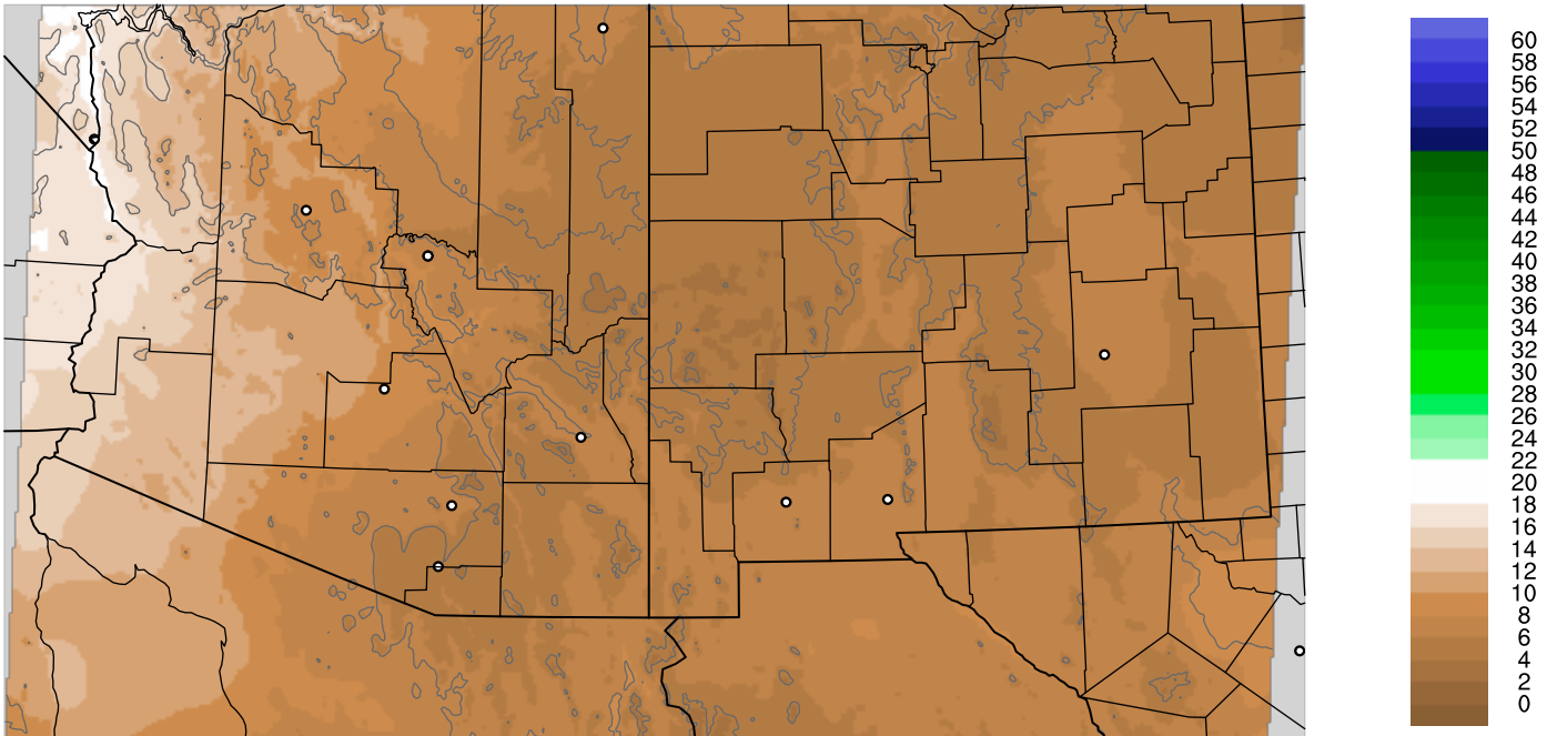
Corrected PWV 9 Jan 2023 17:45 UTC
