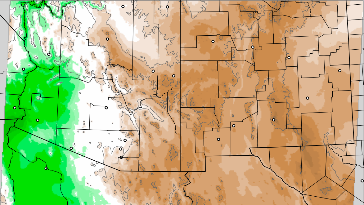
Corrected PWV 12 Sep 2021 11:45 UTC
