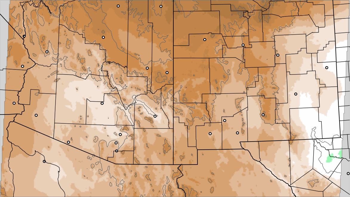
Corrected PWV 22 Nov 2020 11:45 UTC
