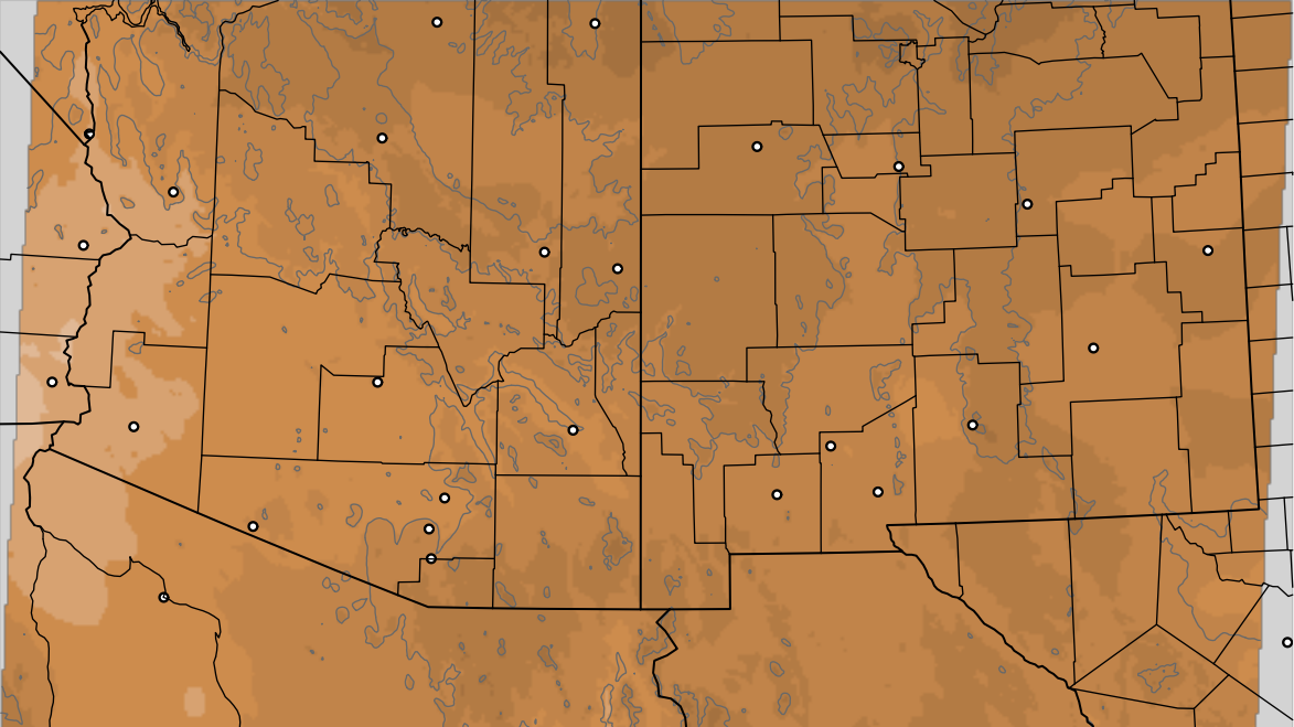
Corrected PWV 12 Nov 2020 11:45 UTC
