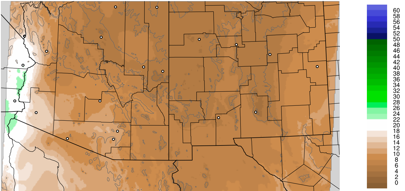
Corrected PWV 8 Oct 2020 11:45 UTC
