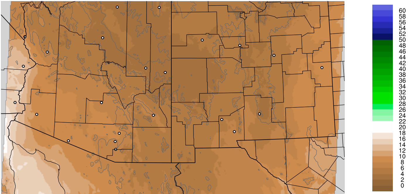
Corrected PWV 7 Oct 2020 11:45 UTC
