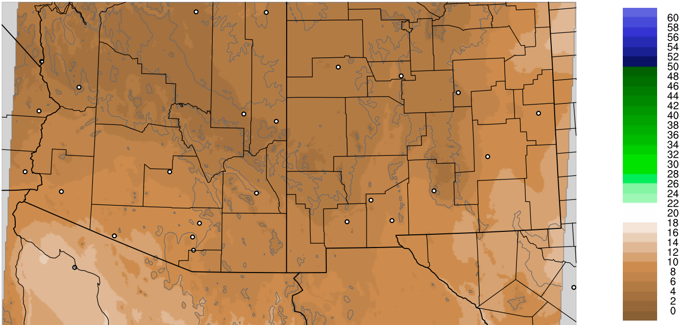
Corrected PWV 3 Oct 2020 11:45 UTC
