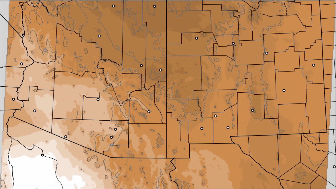
Corrected PWV 29 Sep 2020 11:45 UTC
