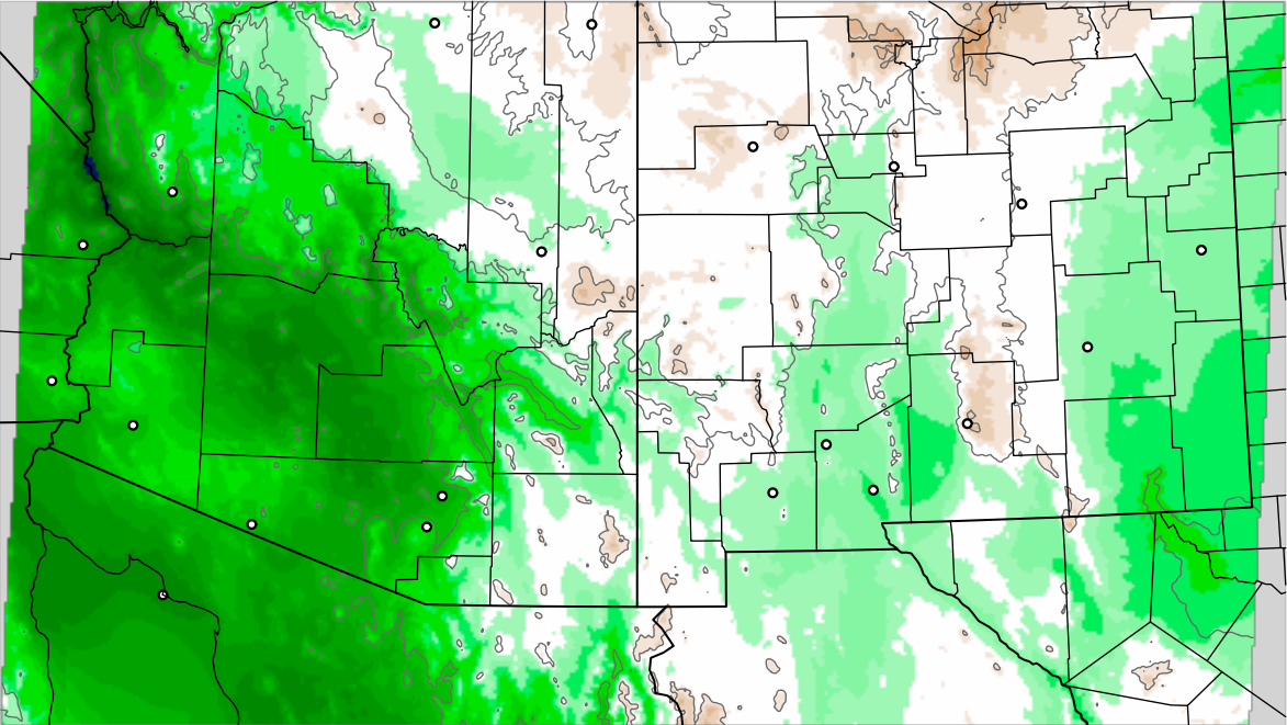
Corrected PWV 23 Aug 2020 11:45 UTC
