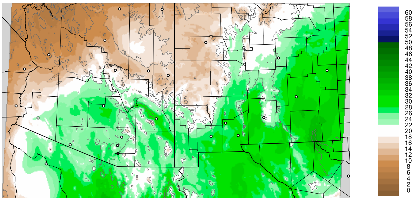
Corrected PWV 8 Aug 2020 11:45 UTC
