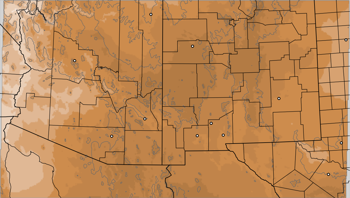
Corrected PWV 10 Jan 2023 11:45 UTC
