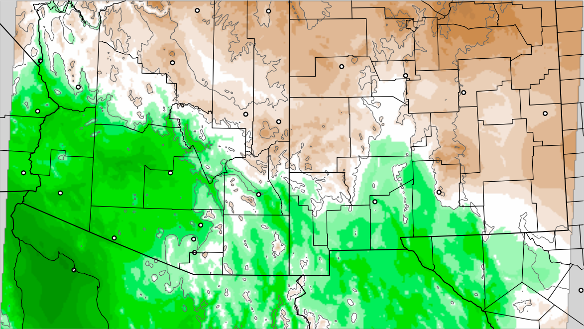
Corrected PWV 24 Sep 2021 11:45 UTC
