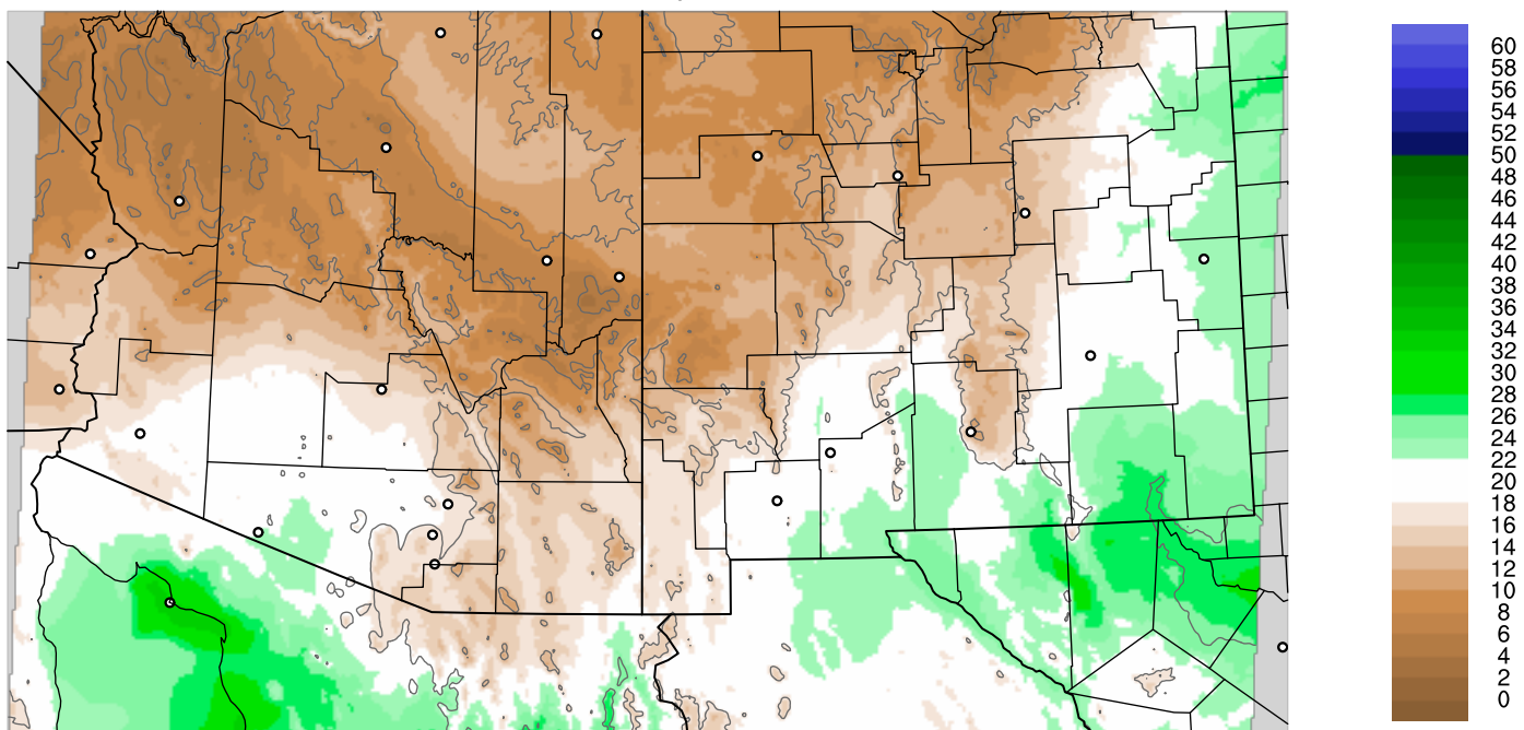
Corrected PWV 16 Sep 2021 8:45 UTC
