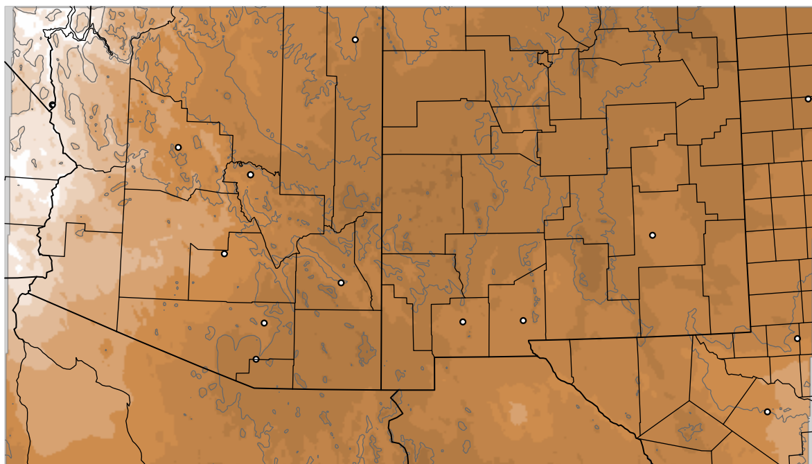
Corrected PWV 9 Jan 2023 17:45 UTC
