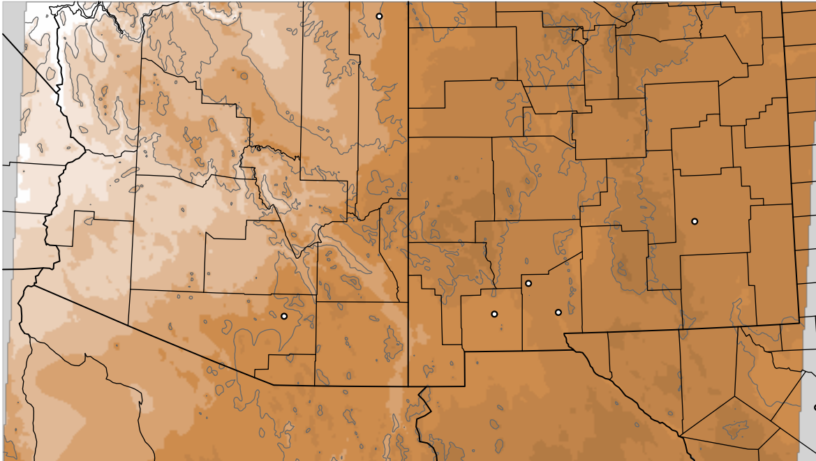
Corrected PWV 9 Jan 2023 23:45 UTC
