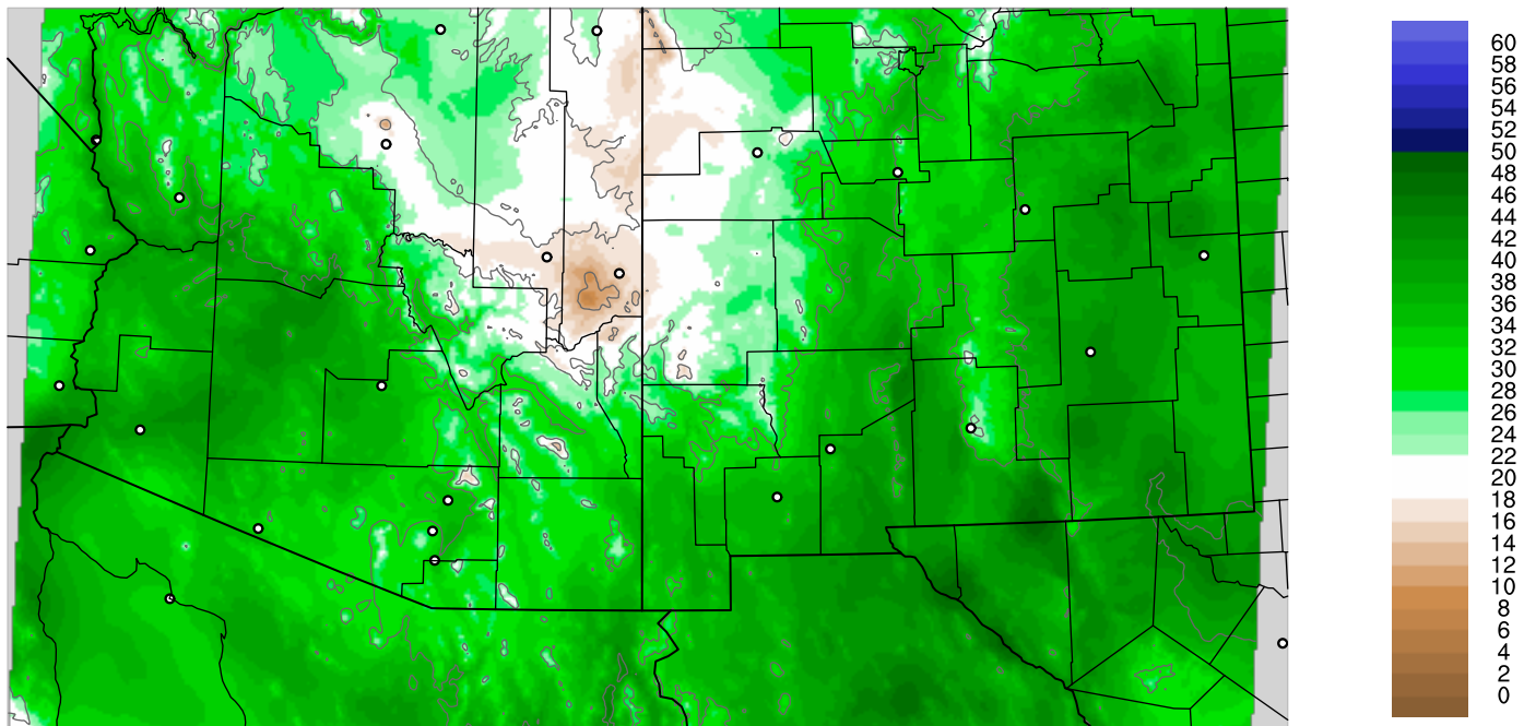
Corrected PWV 1 Sep 2021 23:45 UTC
