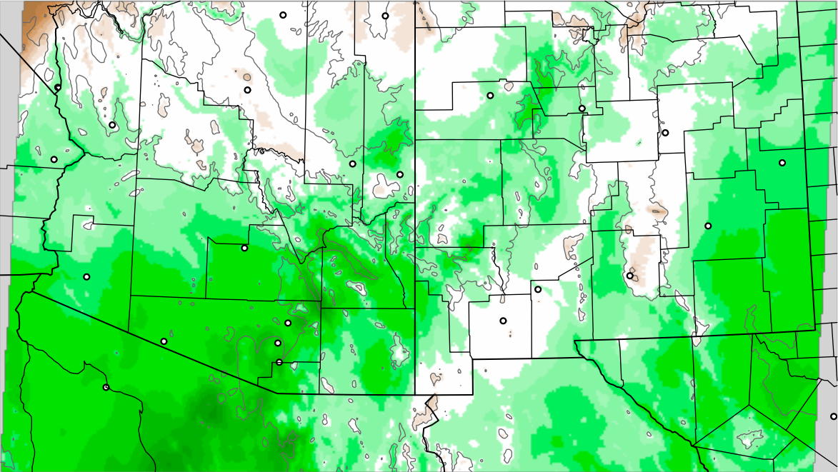
Corrected PWV 26 Aug 2021 23:45 UTC
