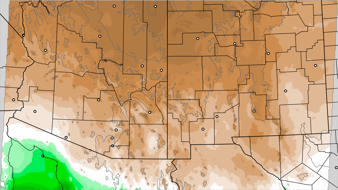
Corrected PWV 21 Sep 2021 23:45 UTC
