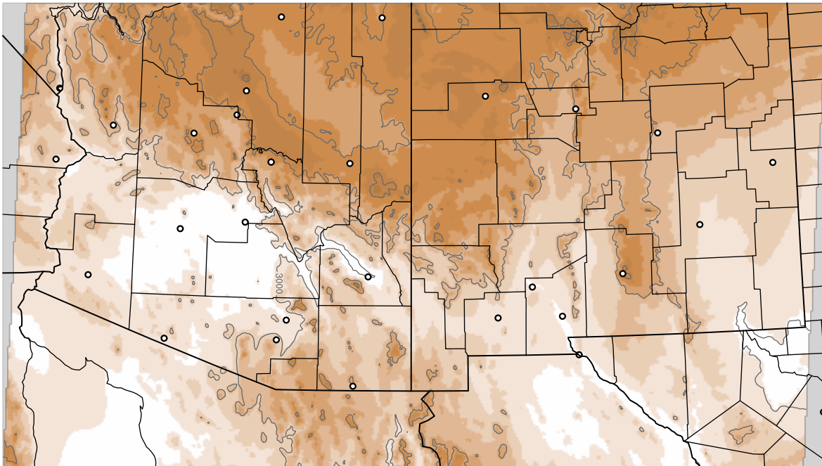
Corrected PWV 8 Dec 2018 5:45 UTC
