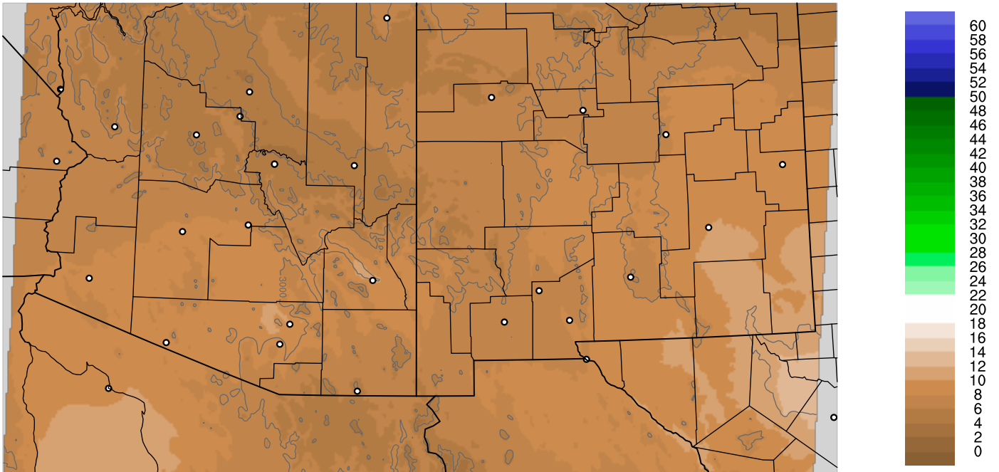
Corrected PWV 5 Dec 2018 5:45 UTC
