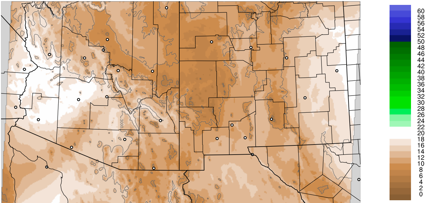
Corrected PWV 17 Oct 2018 5:45 UTC
