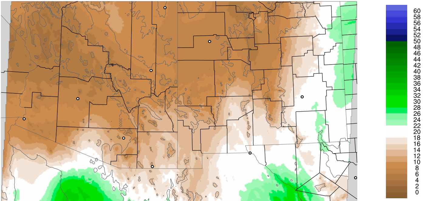
Corrected PWV 27 Jun 2018 5:45 UTC
