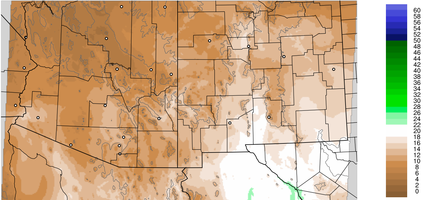
Corrected PWV 18 Oct 2021 5:45 UTC
