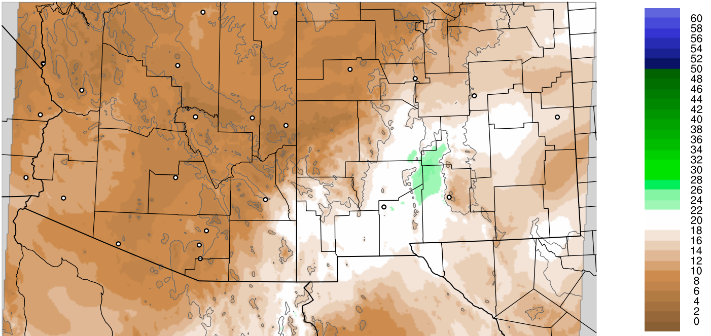
Corrected PWV 10 Oct 2021 5:45 UTC
