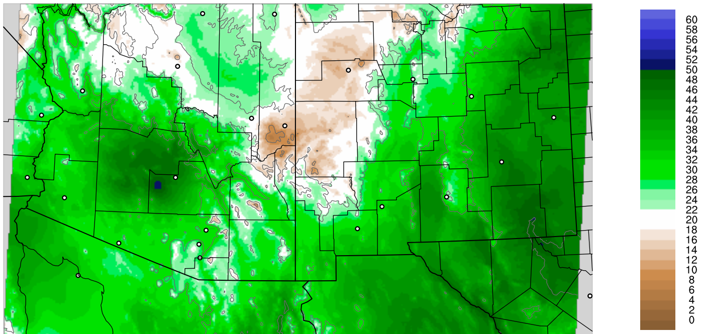
Corrected PWV 2 Sep 2021 5:45 UTC
