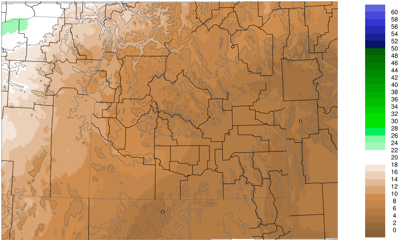
Corrected PWV 18 Jan 2017 5:45 UTC
