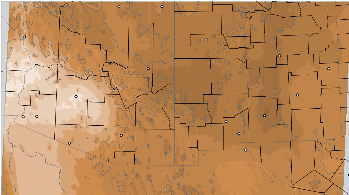
Corrected PWV 12 Jan 2018 11:45 UTC
