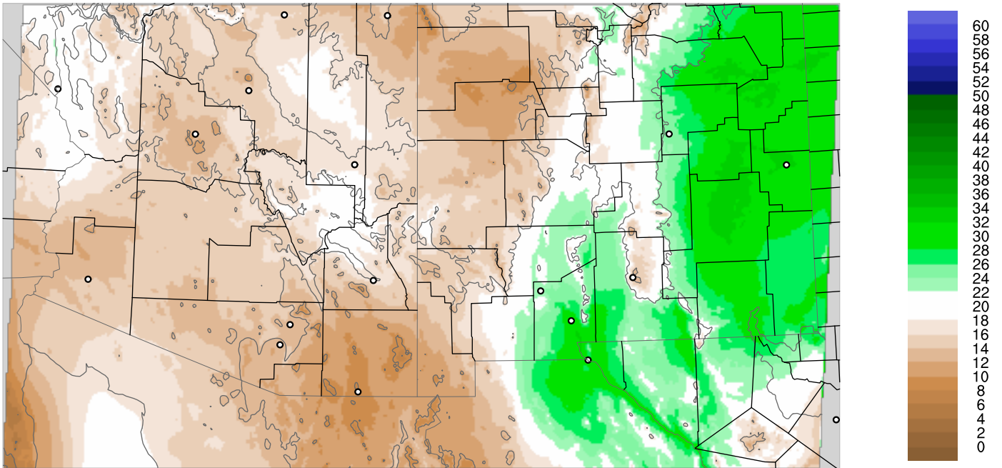
Corrected PWV 19 Jun 2017 11:45 UTC
