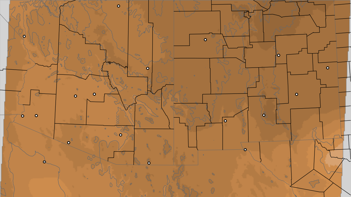
Corrected PWV 20 Nov 2017 11:45 UTC
