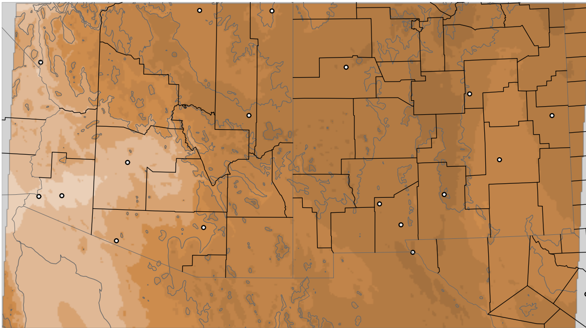
Corrected PWV 11 Jan 2018 23:45 UTC
