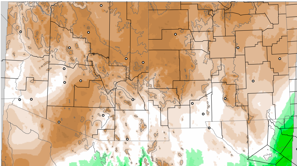
Corrected PWV 21 Sep 2017 5:45 UTC
