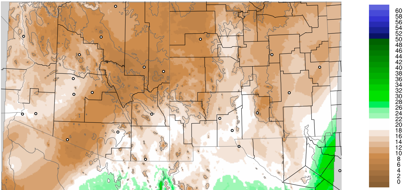
Corrected PWV 21 Sep 2017 5:45 UTC
